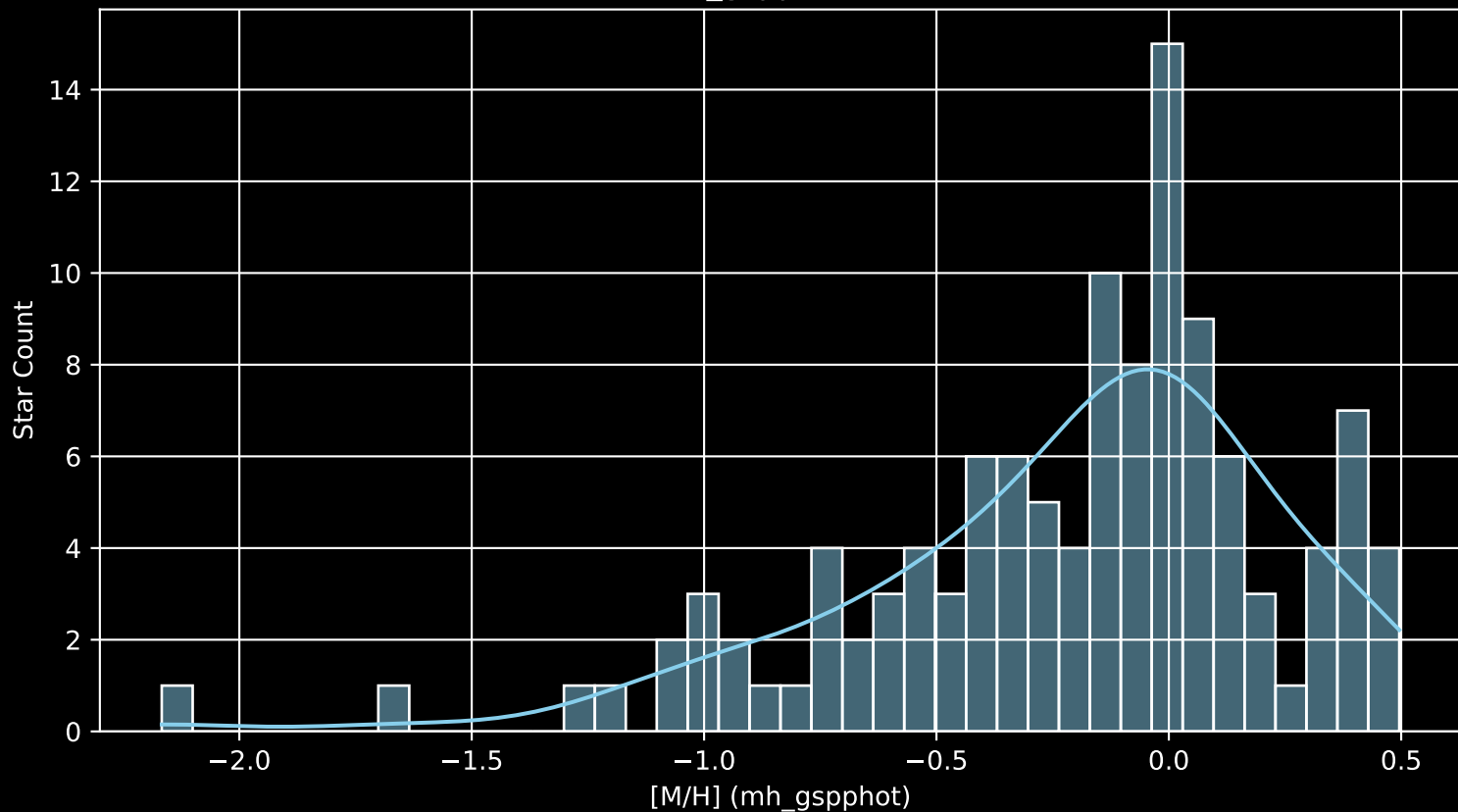
APOGEE DR17 Field: [045+00 [M/H] (mh_gspphot) (n= 117)
