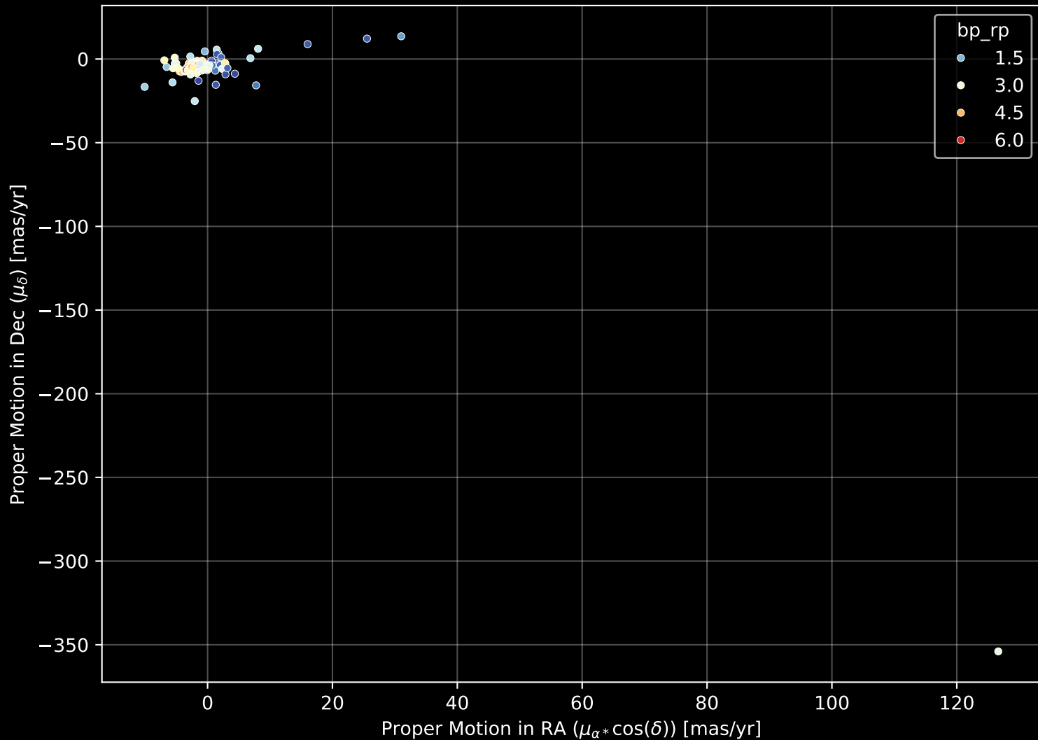
APOGEE DR17 Field: [045+00] Proper Motion Diagram (n= 130)
