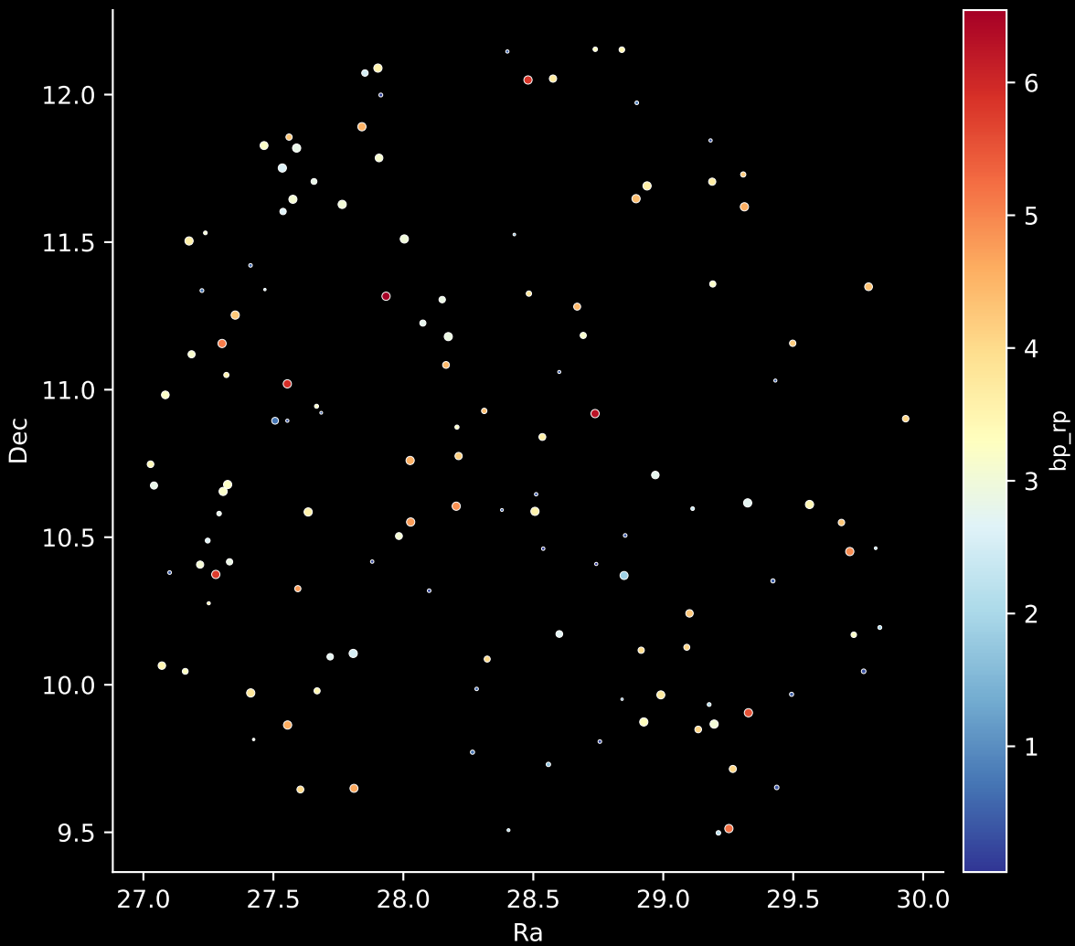
APOGEE DR17 Field: [045+00] Stars: 130
