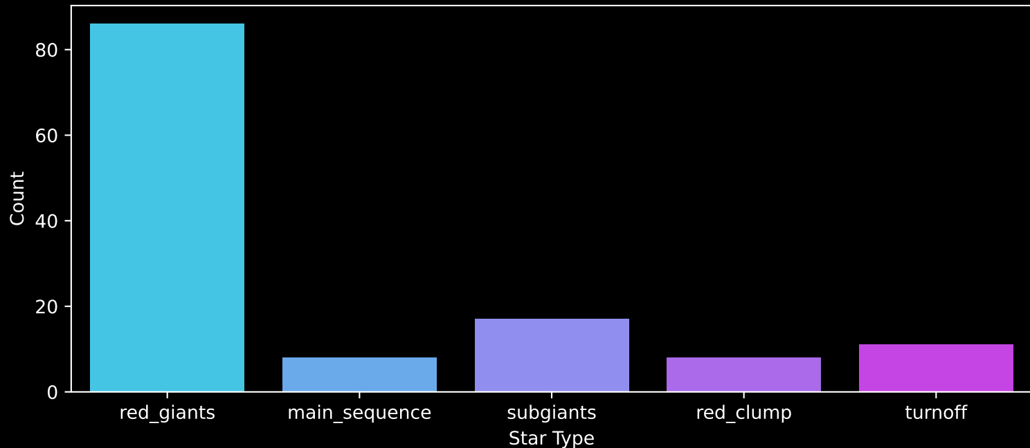
APOGEE DR17 Field: [045+00] Count plot of Star Type
