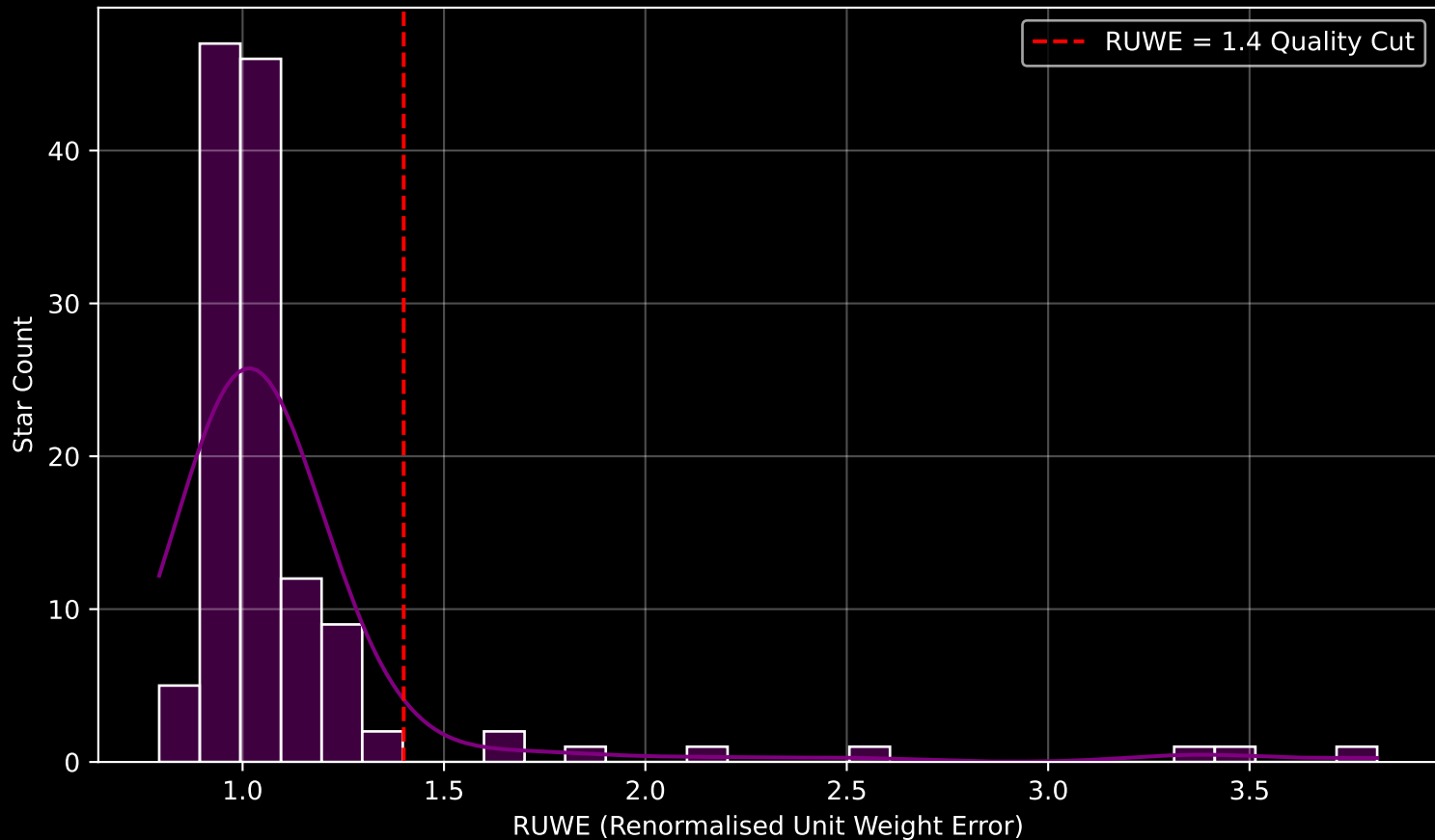
GAPOGEE DR17 Field [045+00] RUWE Distribution (n= 129)
