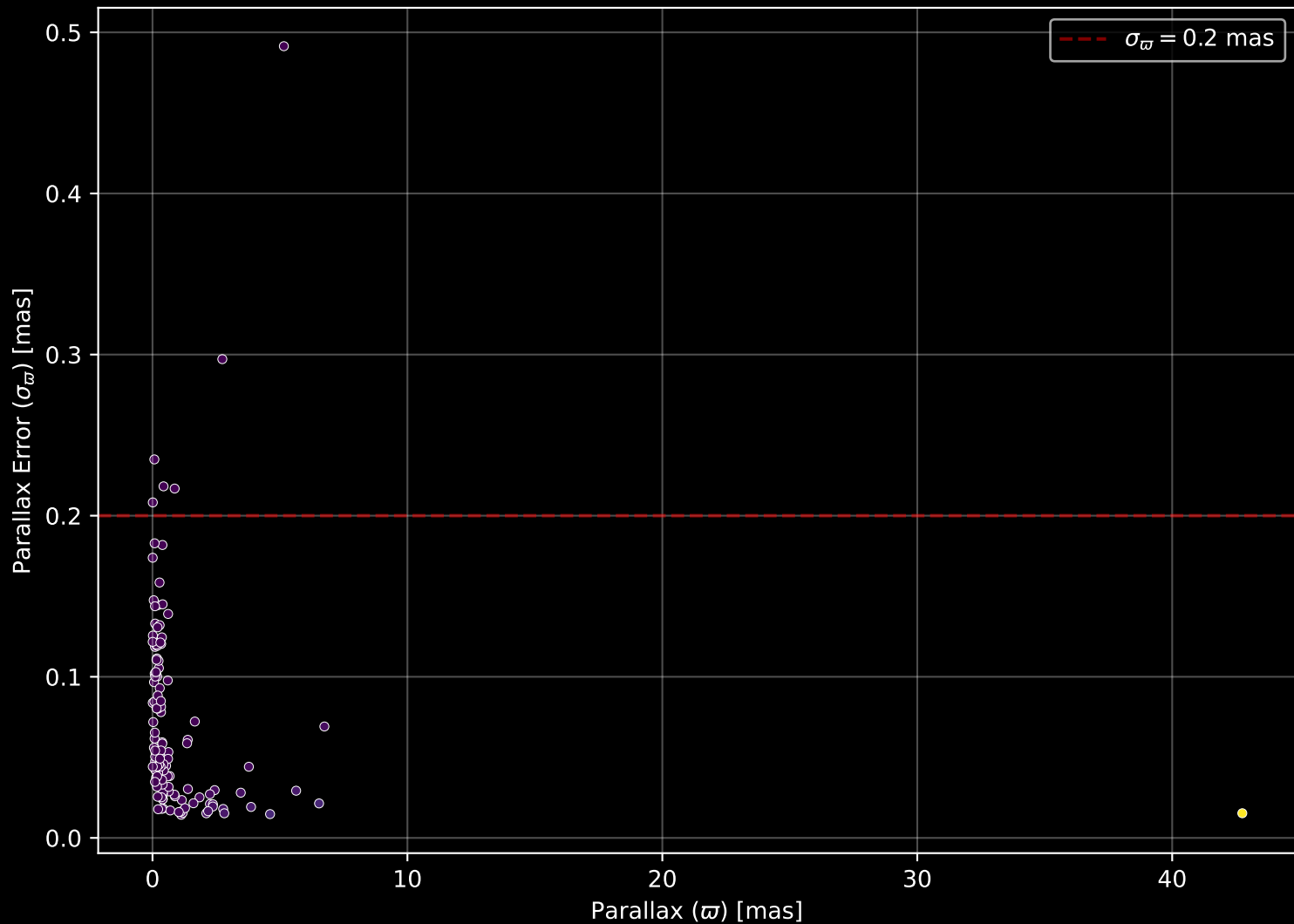
APOGEE DR17 Field: [045+00] Parallax Quality (n= 130)
